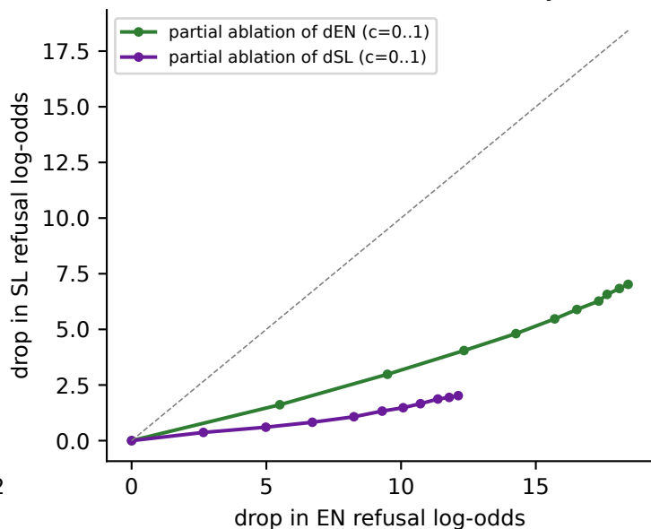
Gemma-3-12B-it: matched-efficacy curves
