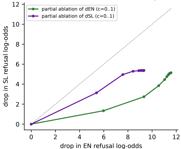
GaMS3-12B-Instruct: matched-efficacy curves
