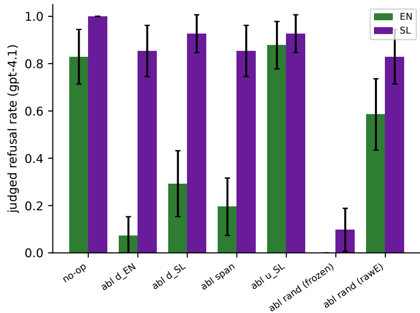
Gemma-3-12B-it: harmful half-B prompts
