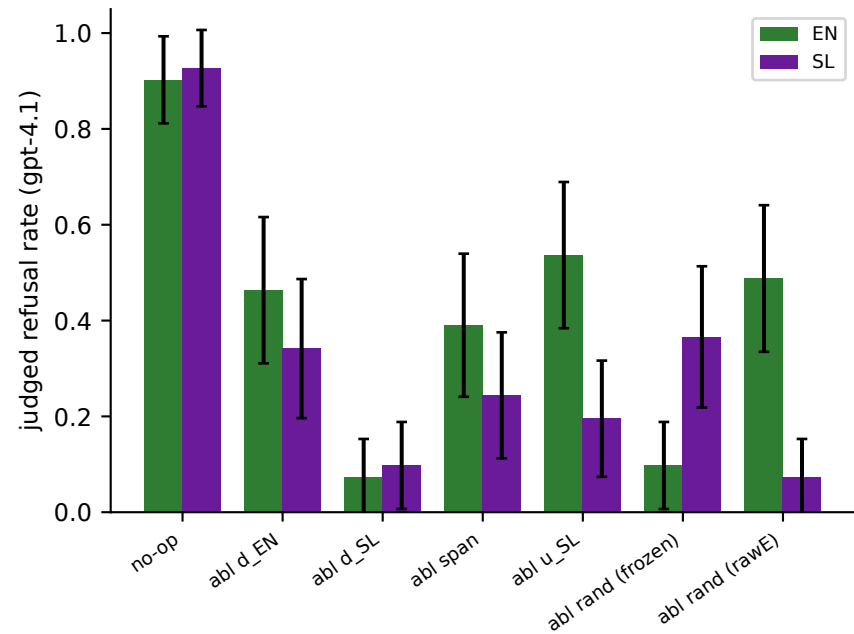
GaMS3-12B-Instruct: harmful half-B prompts
