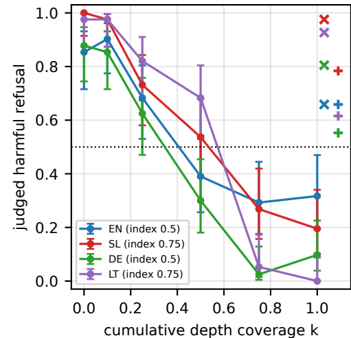
Depth-coverage curves (x = single site h^* , + = matched random at full depth)
