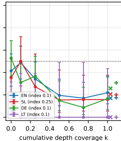
Depth-coverage curves (x = single site h^* , + = matched random at full depth)
