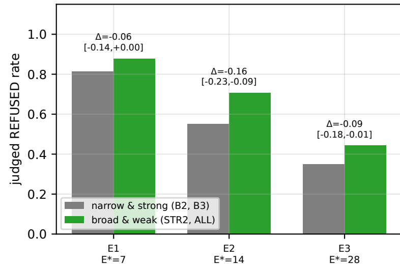
SL harmful refusal
