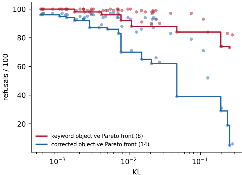
Identical 60 startup edits, two objectives
