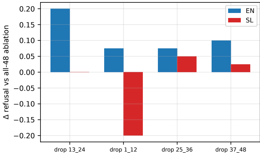
Leave-one-band-out necessity (higher = band is needed)
