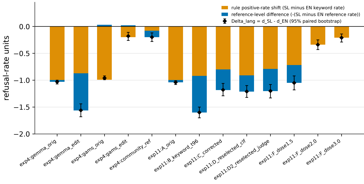
Language dependence of the keyword discrepancy on 100 verified EN-SL pairs (Qwen3-14B reference)
