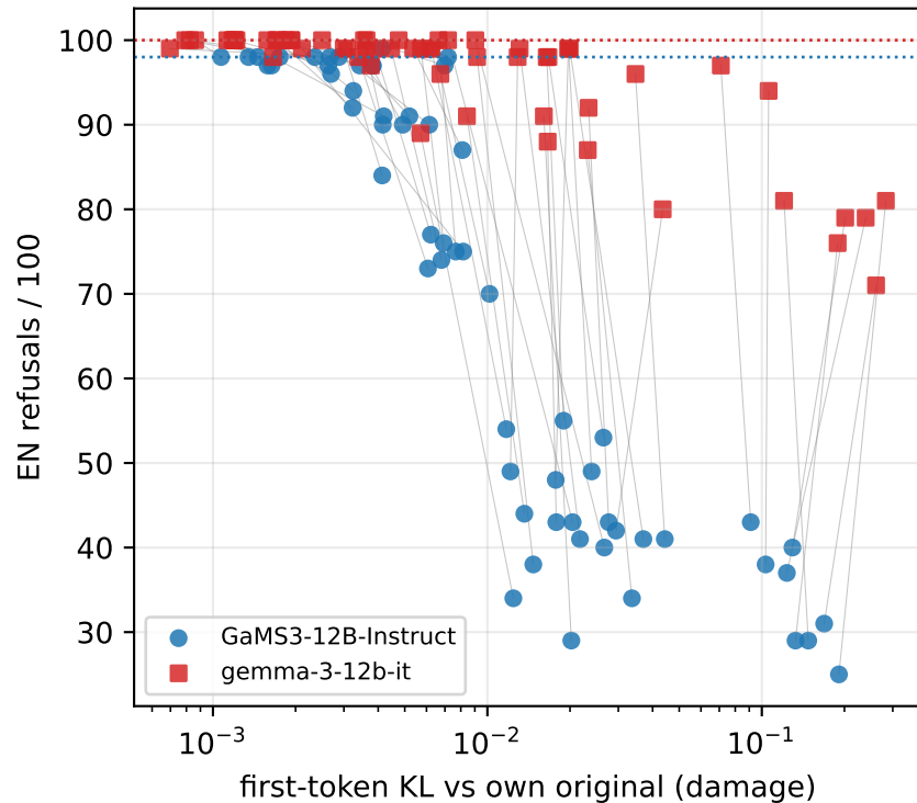
Same 60 edits, both models (grey lines join one identical edit)
