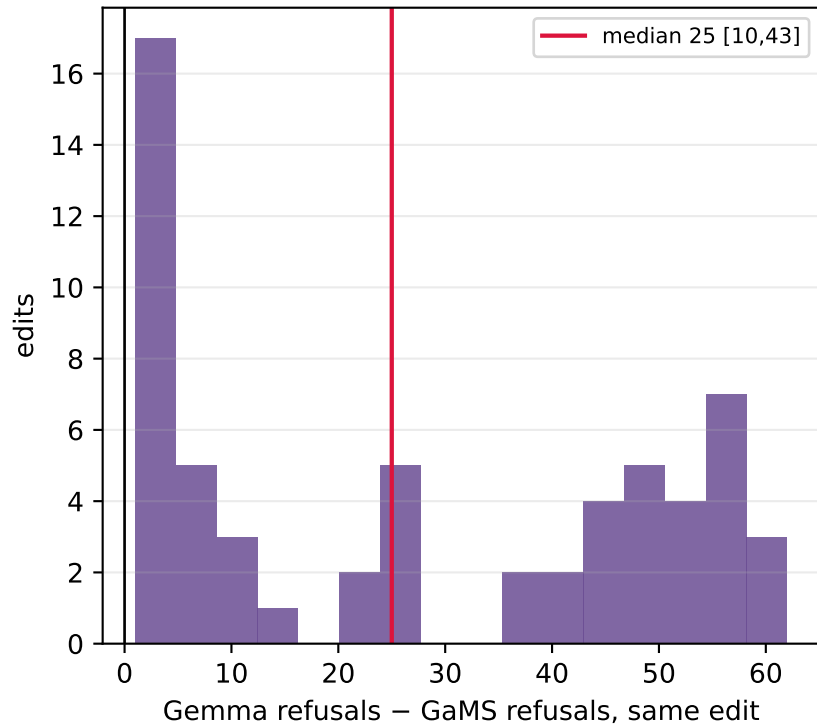
60/60 edits: Gemma refuses more efficiency gap \times 13.4 [6.9,30.4]
