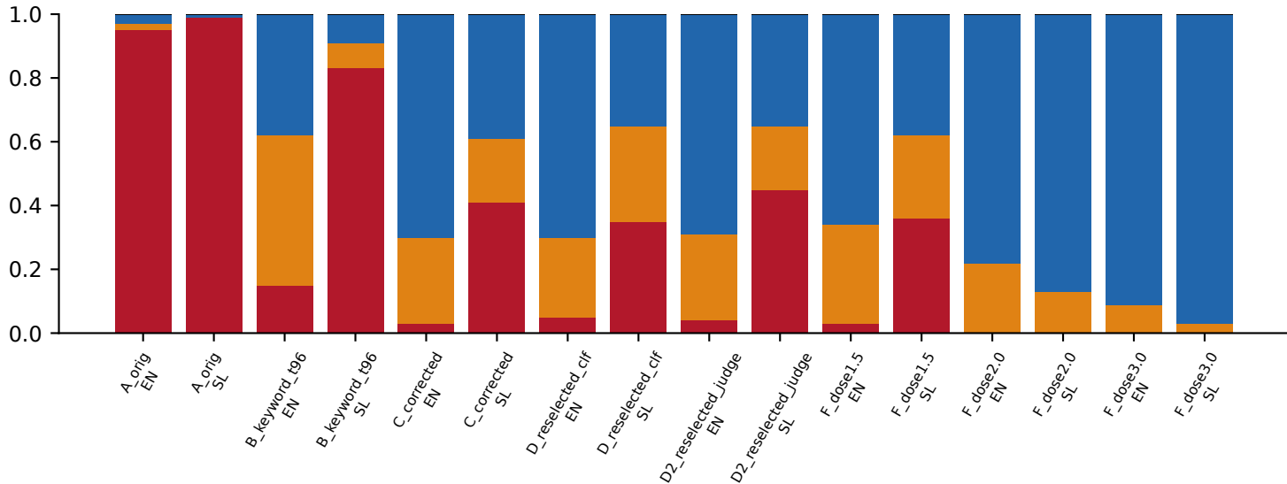
share of S5X responses (Qwen3-14B)
