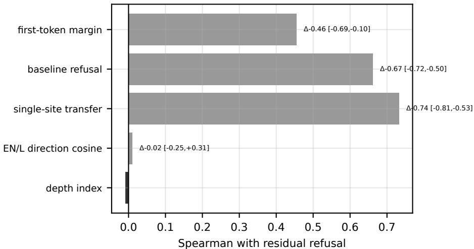
Predictor comparison (CI = paired item bootstrap on the difference vs index)
