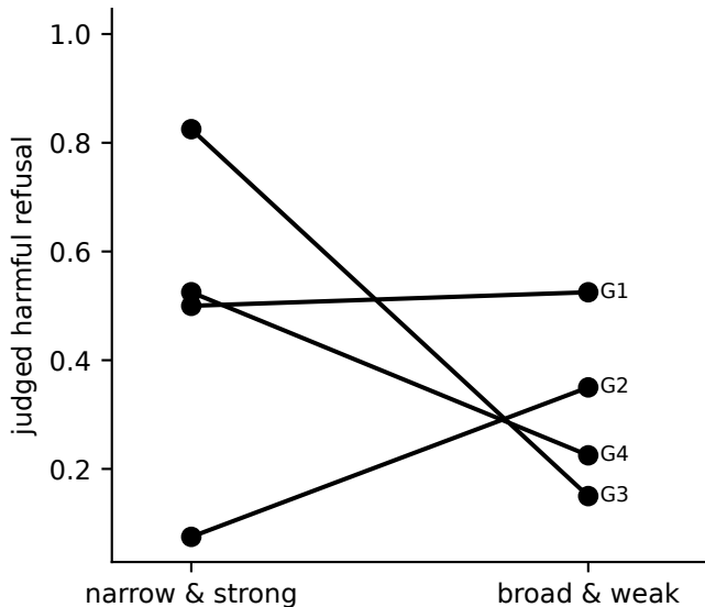
EN: matched-energy pairs (screen)
