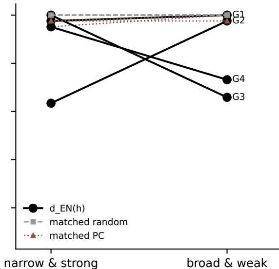
SL: matched-energy pairs (screen)
