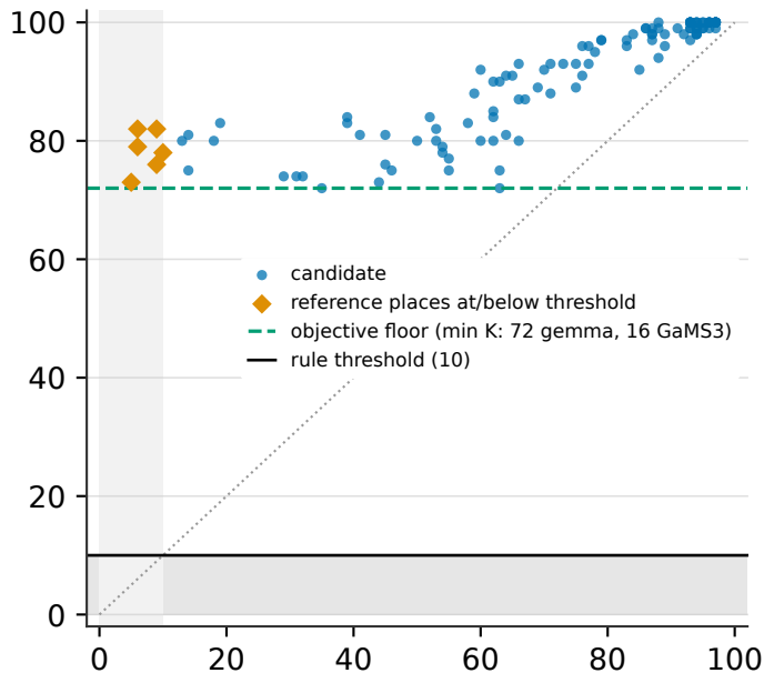
keyword objective K / 100
