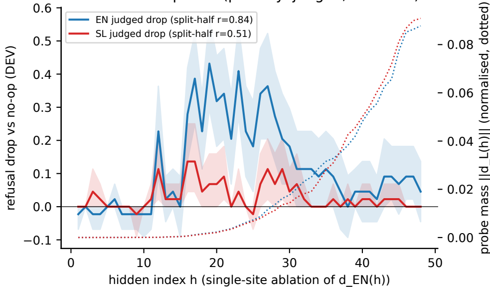
Causal write profile (primary: judged, PRIMARY)
