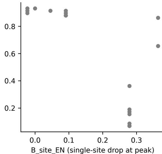
B_site: \rho=-0.78
