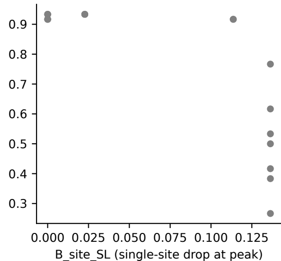
B_site: \rho=-0.79
