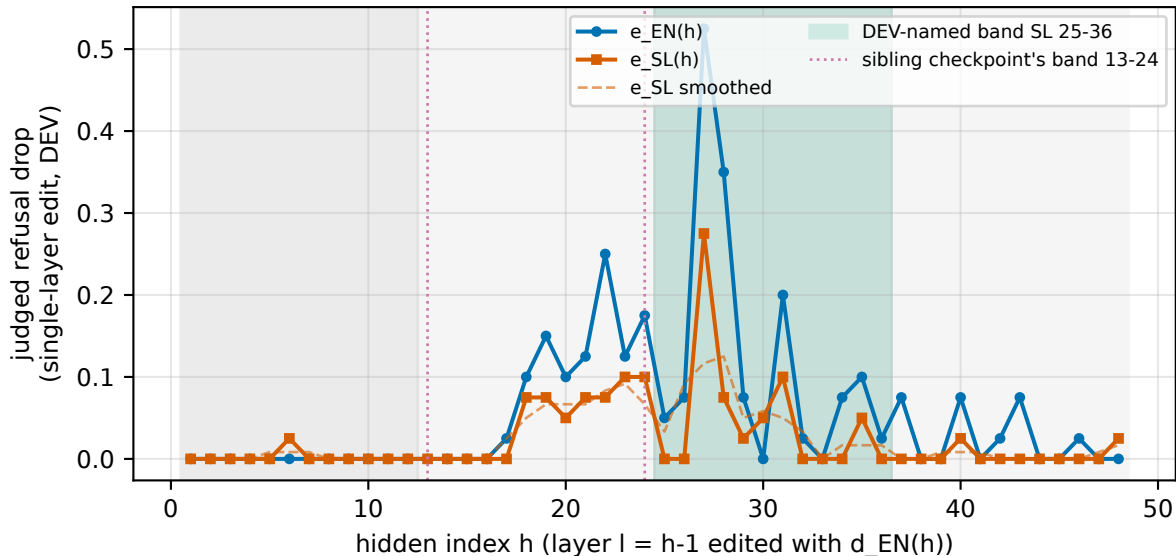
Causal write profile of the refusal edit, GaMS3-12B-Instruct (c = 2.5)
