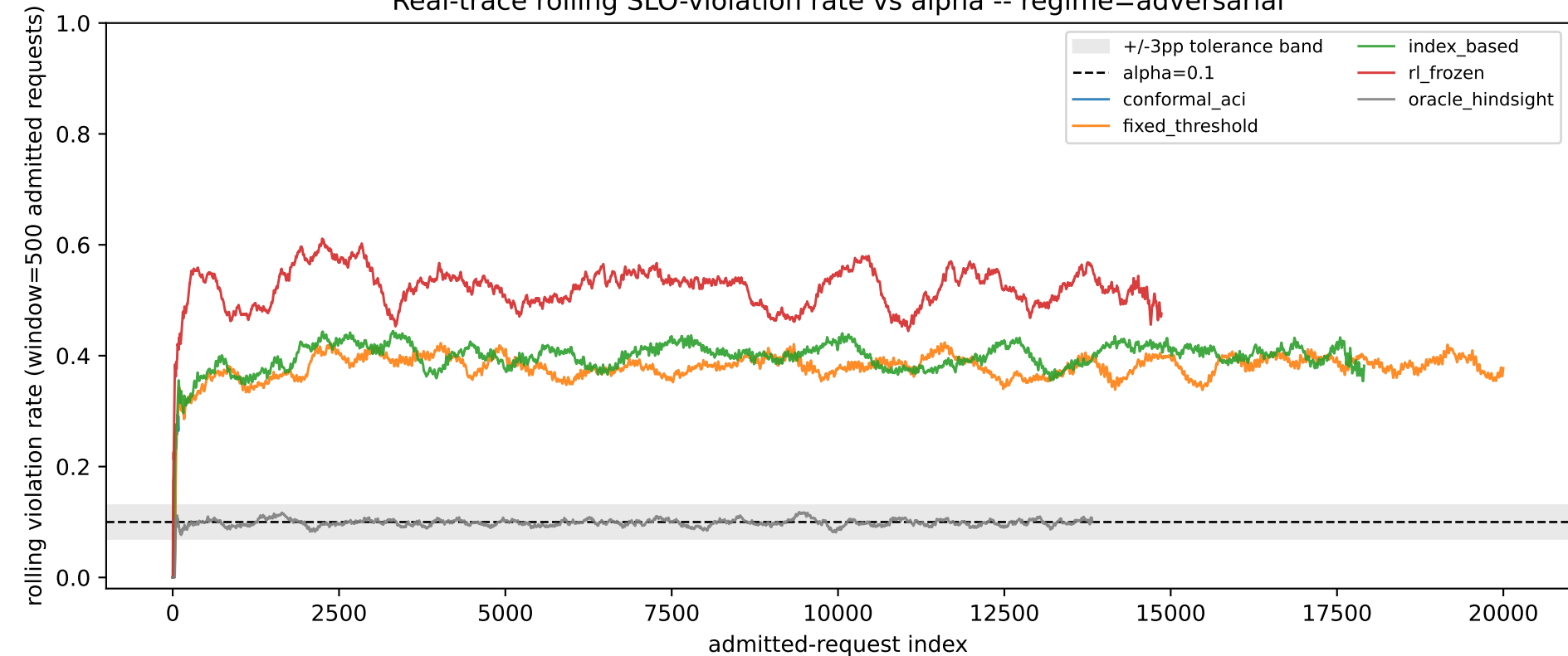
Real-trace rolling SLO-violation rate vs alpha -- regime=adversarial
