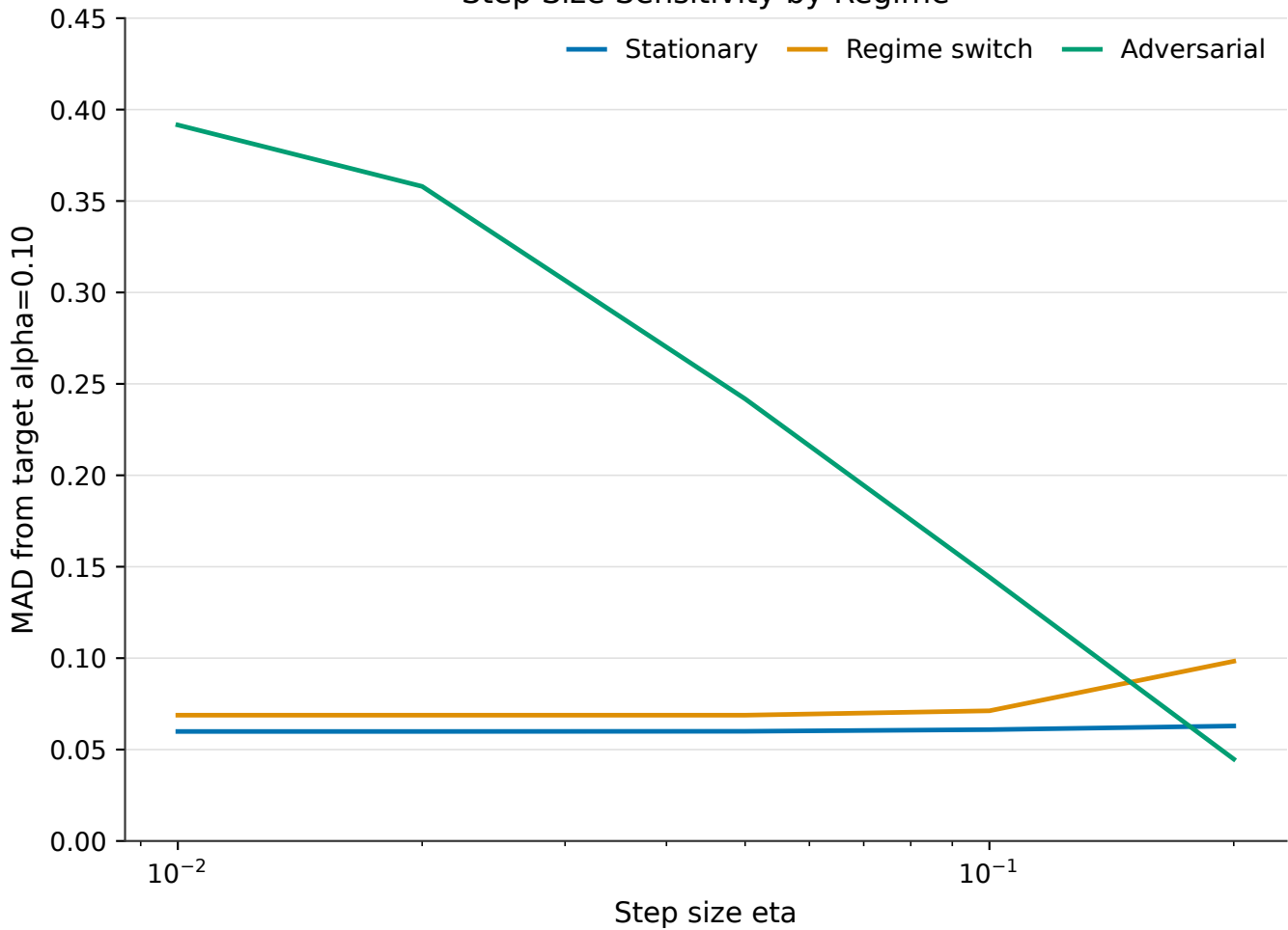
Step Size Sensitivity by Regime
