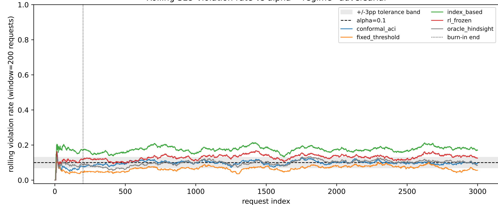
Rolling SLO-violation rate vs alpha -- regime=adversarial
