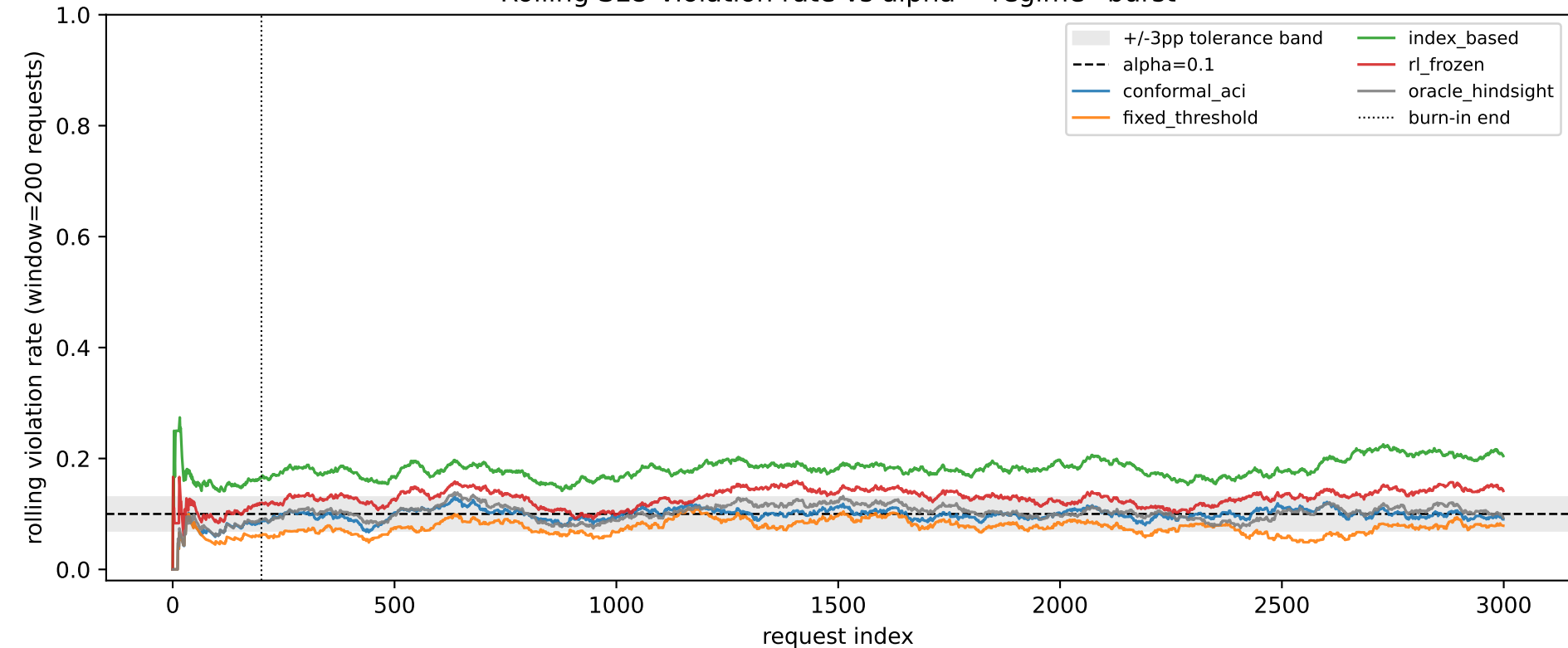
Rolling SLO-violation rate vs alpha -- regime=burst
