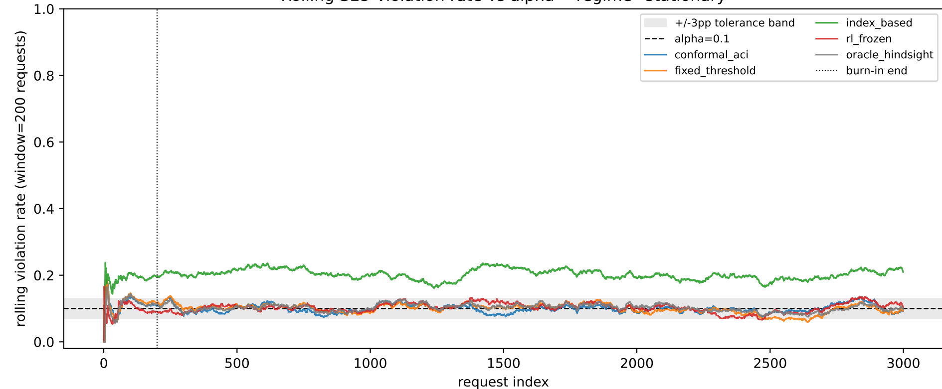
Rolling SLO-violation rate vs alpha -- regime=stationary
