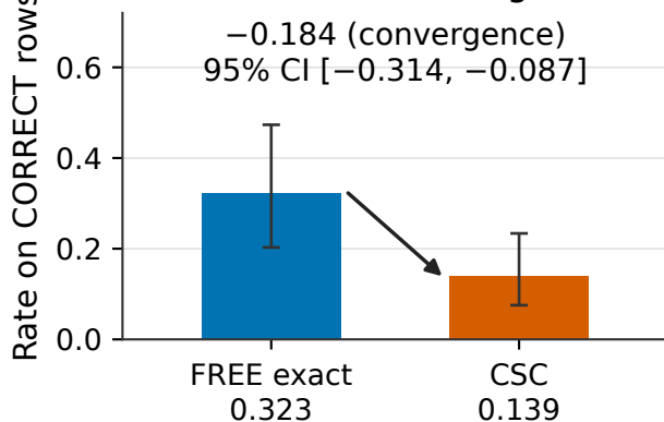
(b) Correct-row divergence d
