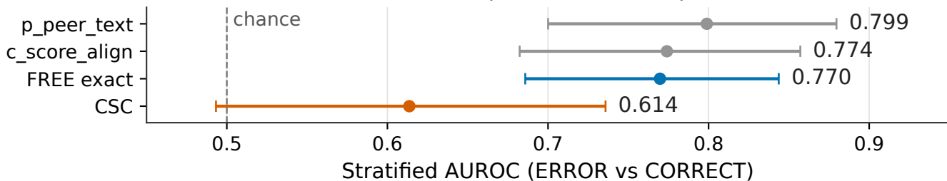
(c) Discriminative power on development set E
