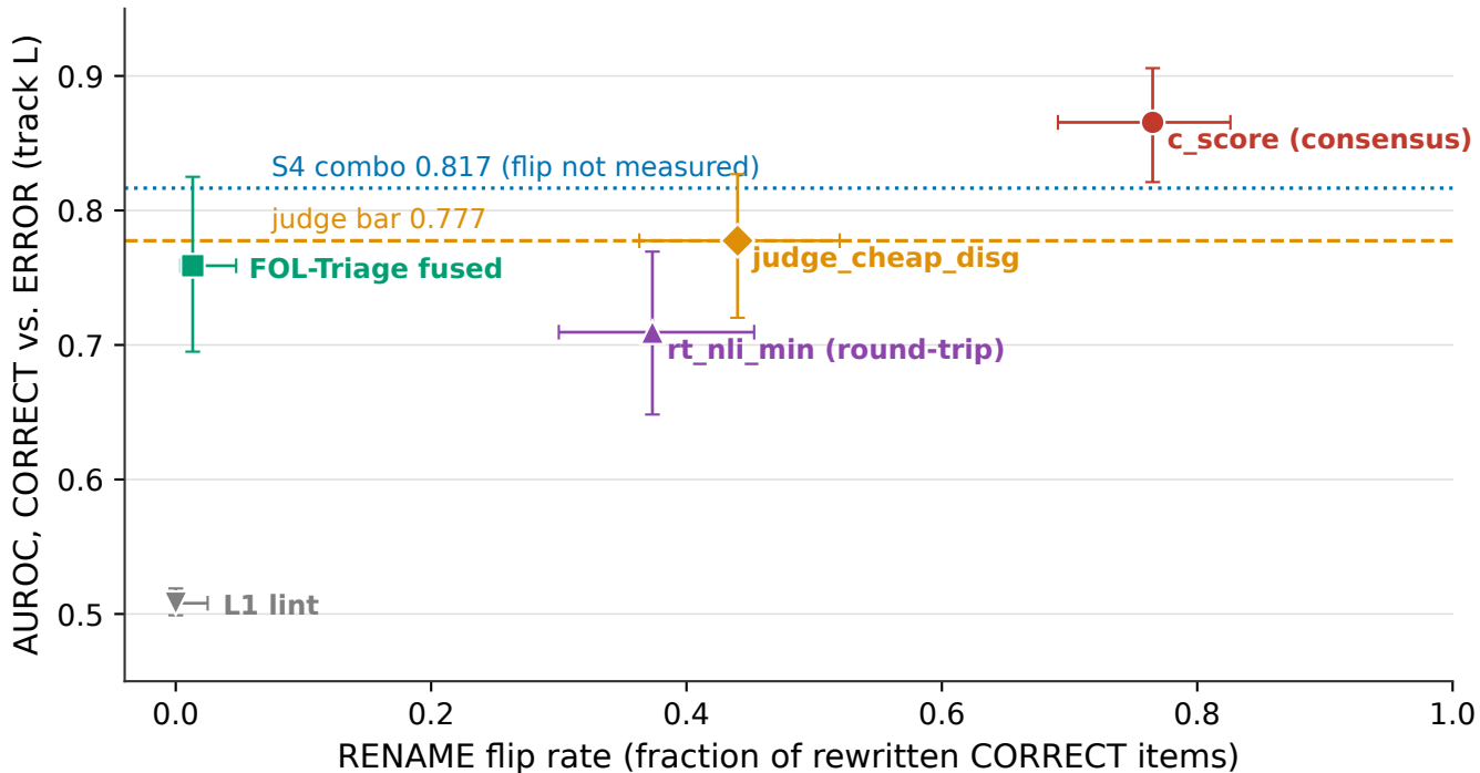
Iteration 1: error detection vs. rename invariance
