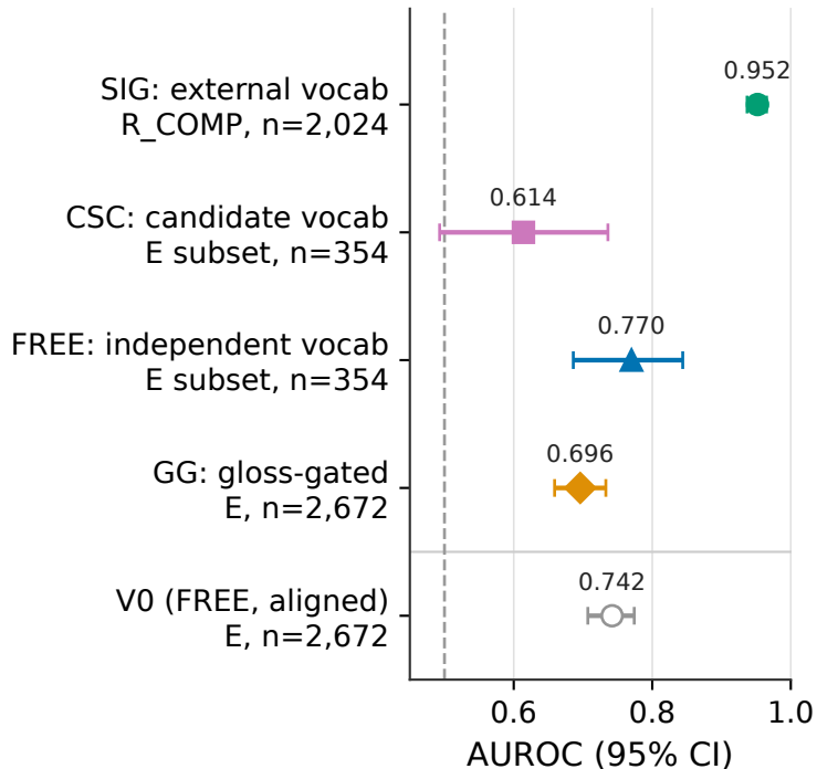
(b) Discrimination
