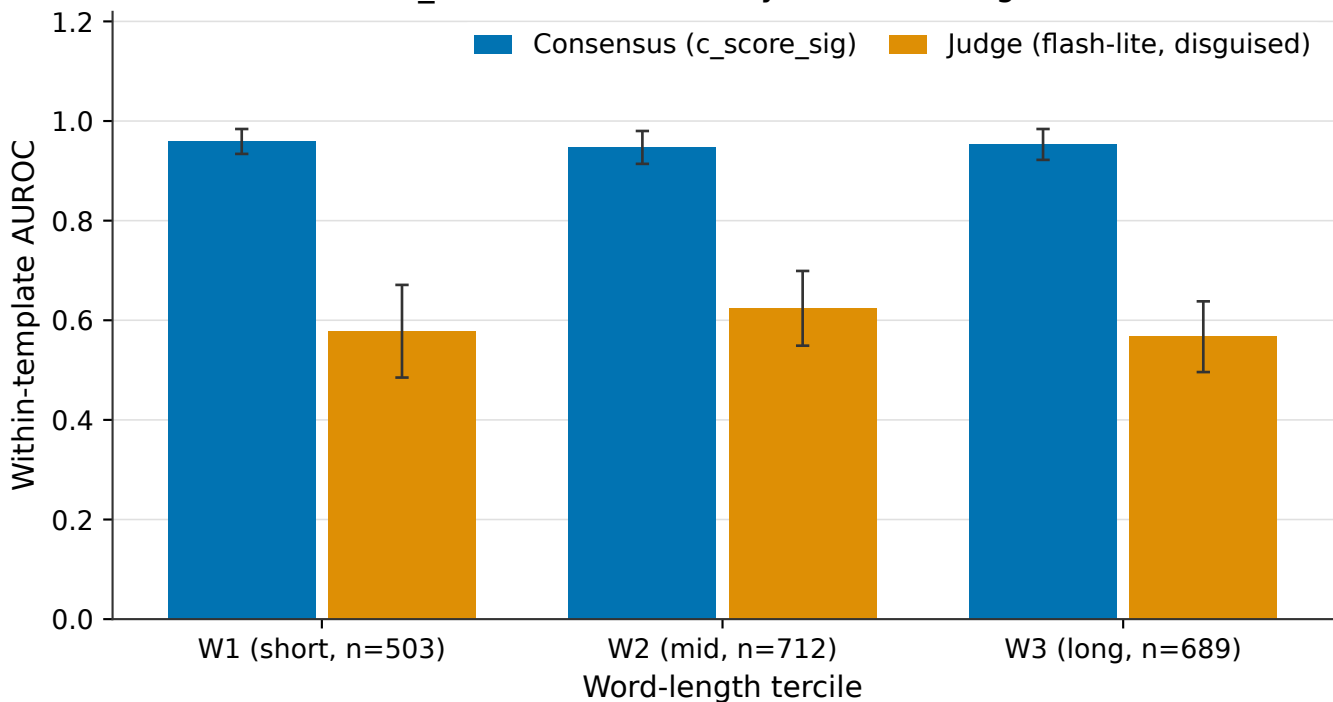
R_COMP-SIG: AUROC by sentence length
