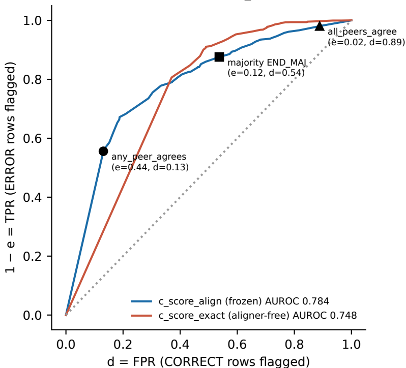
Graded consensus ROC ( R_{AB} , n=2,672 )
