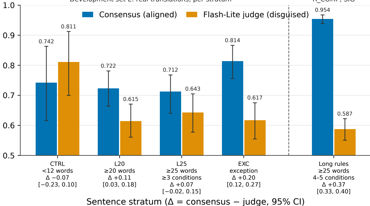
Development set E: real translations, per stratum
