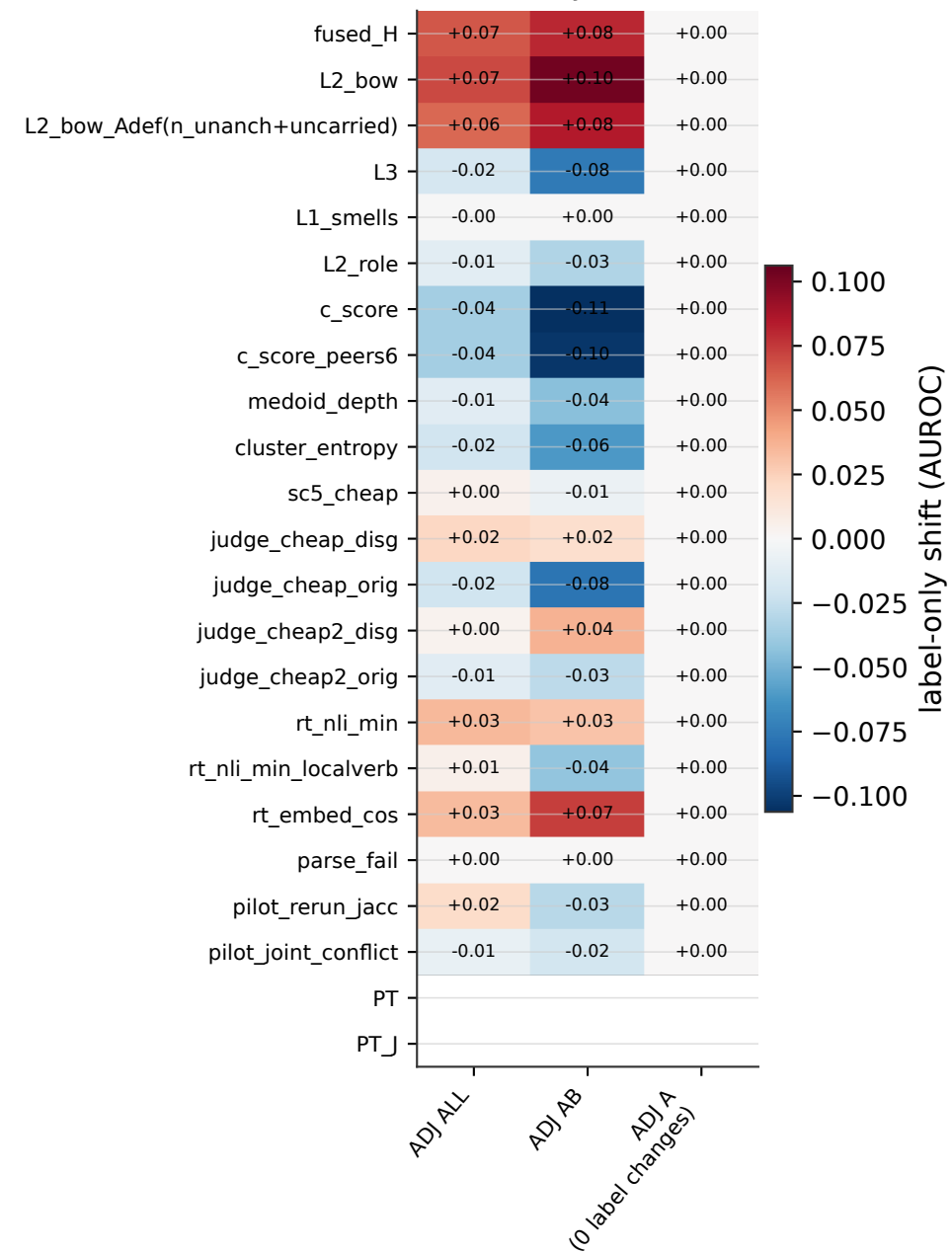
b Label-only shift vs solver labels
