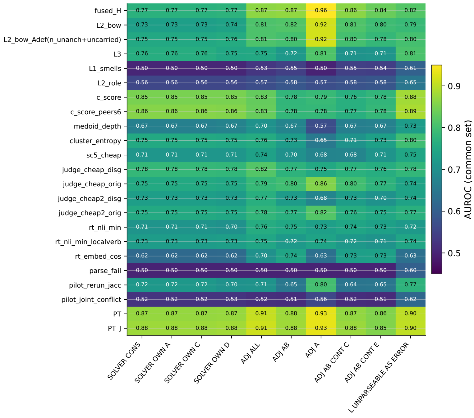
a Common-set AUROC by label regime
