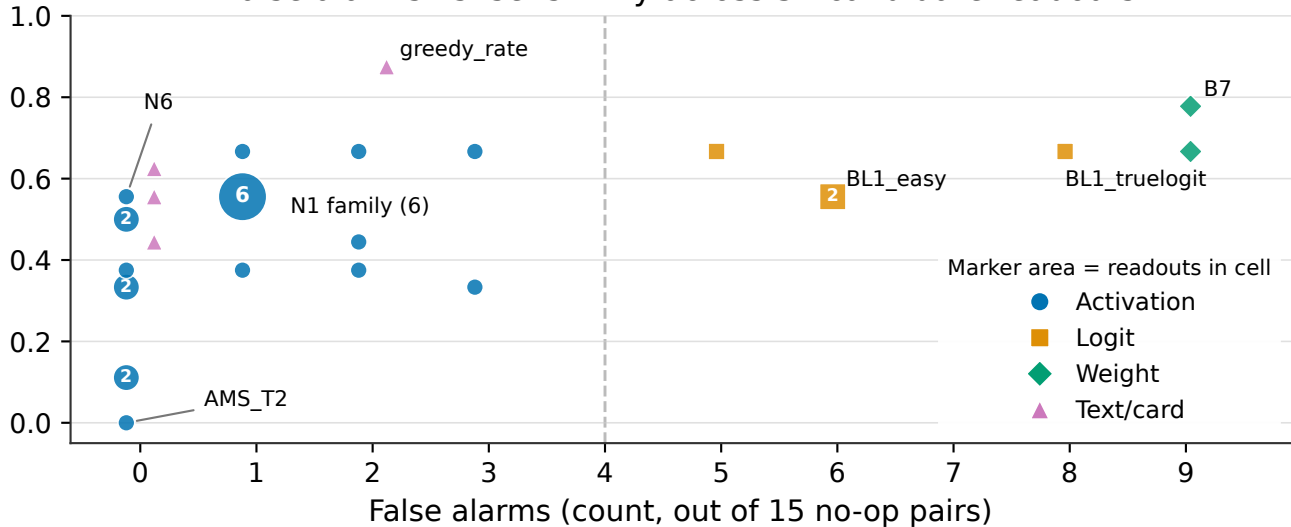
False alarms vs. sensitivity across 32 candidate readouts
