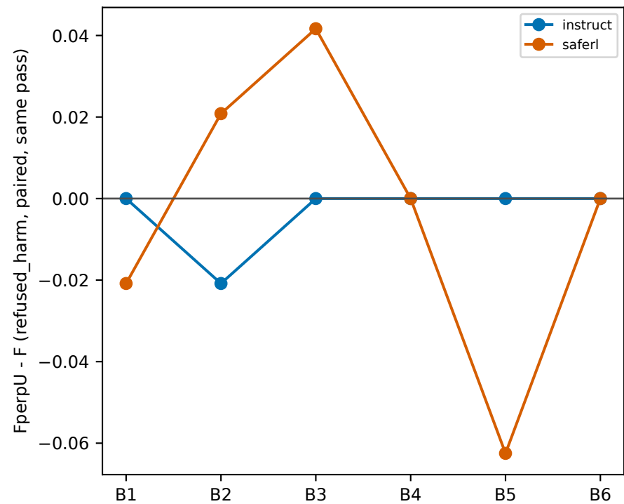
genU (exploratory): does refusal survive removing FperpU?
