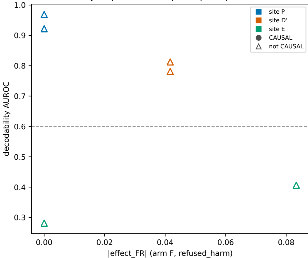
Decodability vs |causal effect| (one point per model x cell)
