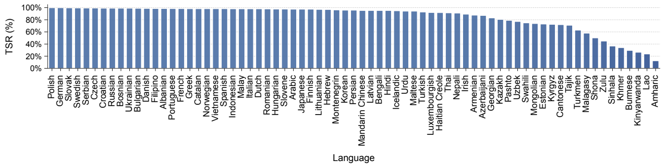
Figure 18: Translation Success Rate (TSR) for semantic preservation across languages.
