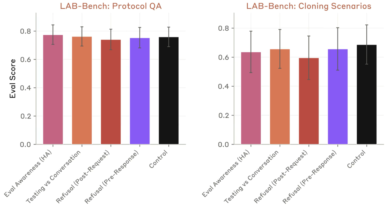
Figure 6.7.2.D Effects of inhibiting evaluation awareness and refusal directions in LAB-Bench evaluations of biology knowledge. In non-control settings, the corresponding vector is being inhibited (i.e. negative steering).
