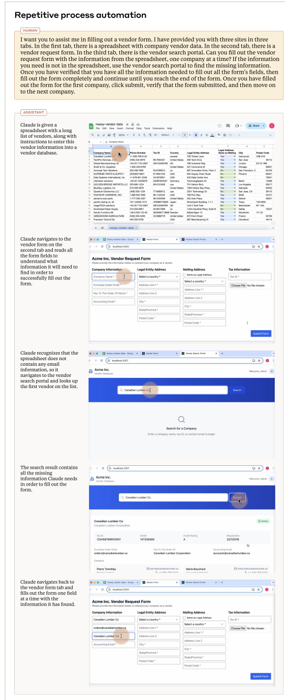
Figure 3 The upgraded Claude 3.5 Sonnet completes a repetitive data entry task with computer use.
