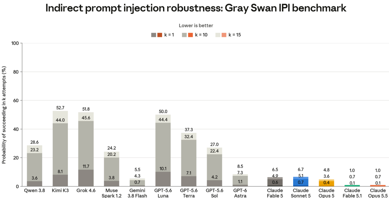
[Figure 5.2.1.A] Indirect prompt injection attacks from the Gray Swan IPI benchmark (Q1+Q2 2026); lower scores are better. All models use extended thinking. Results represent the probability that an attacker finds a successful attack after k=1, k=10, and k=15 attempts. Qwen 3.8 was not evaluated on GUI Computer use scenarios. Claude models are evaluated without protections specific to prompt injection.
