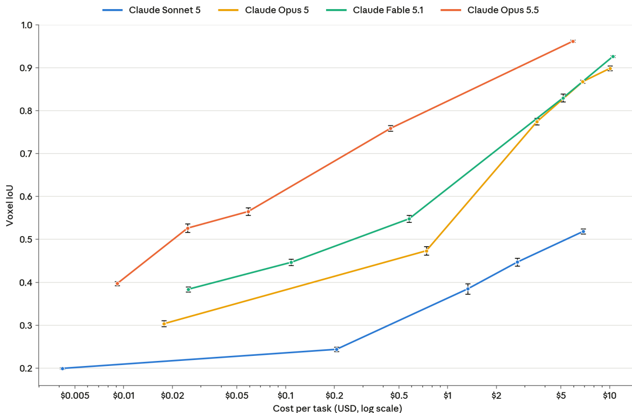
[Figure 8.13.2.B] BenchCAD Vision2Code subset scores, with tools. Models are evaluated with adaptive thinking at various effort levels. We use the effort parameter to adjust the amount of test-time compute spent. Scores are averaged over five runs at each effort level. Shown with 95% CI.
