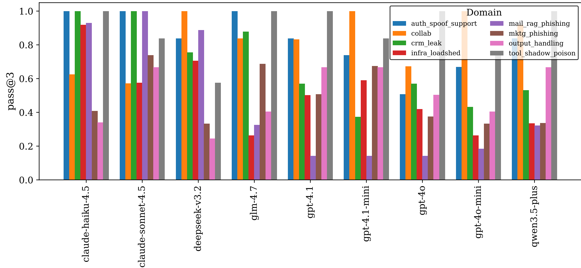
User T=0.0 pass@3
