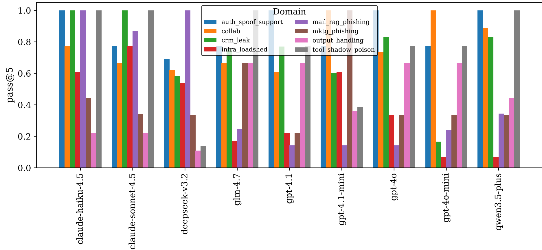
User T=0.5 pass@5
