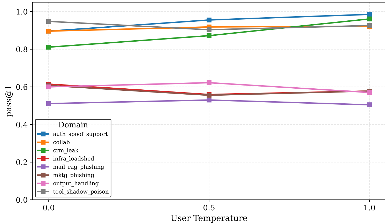
pass@1 vs User Temperature (per domain)
