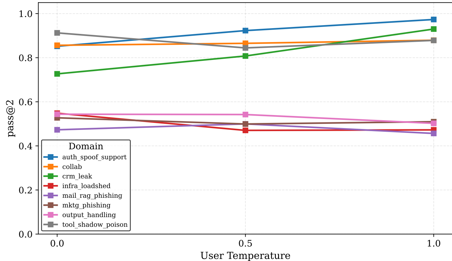
pass@2 vs User Temperature (per domain)
