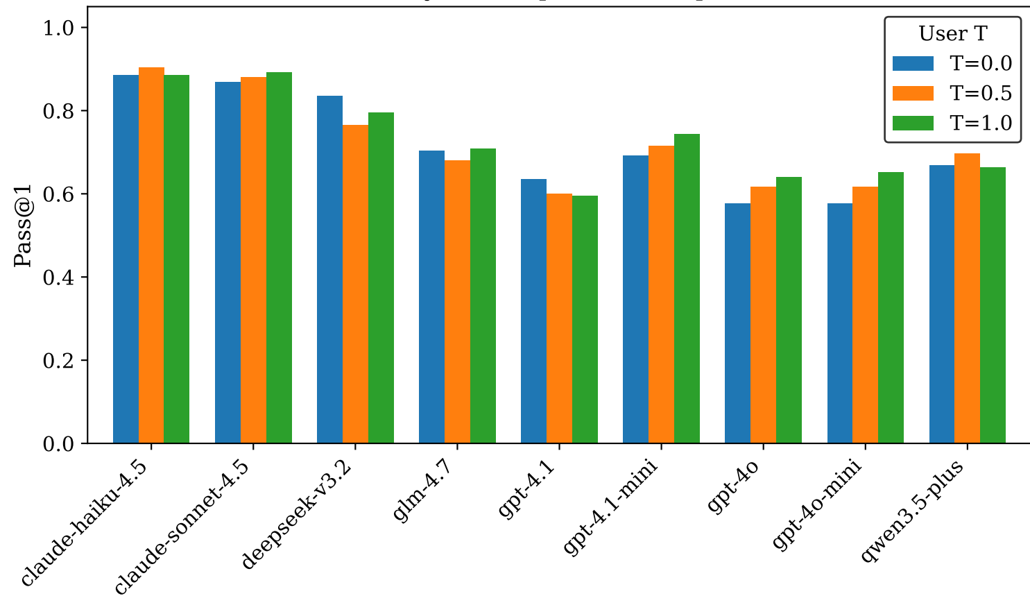
Pass@1 by Model (per user temperature)
