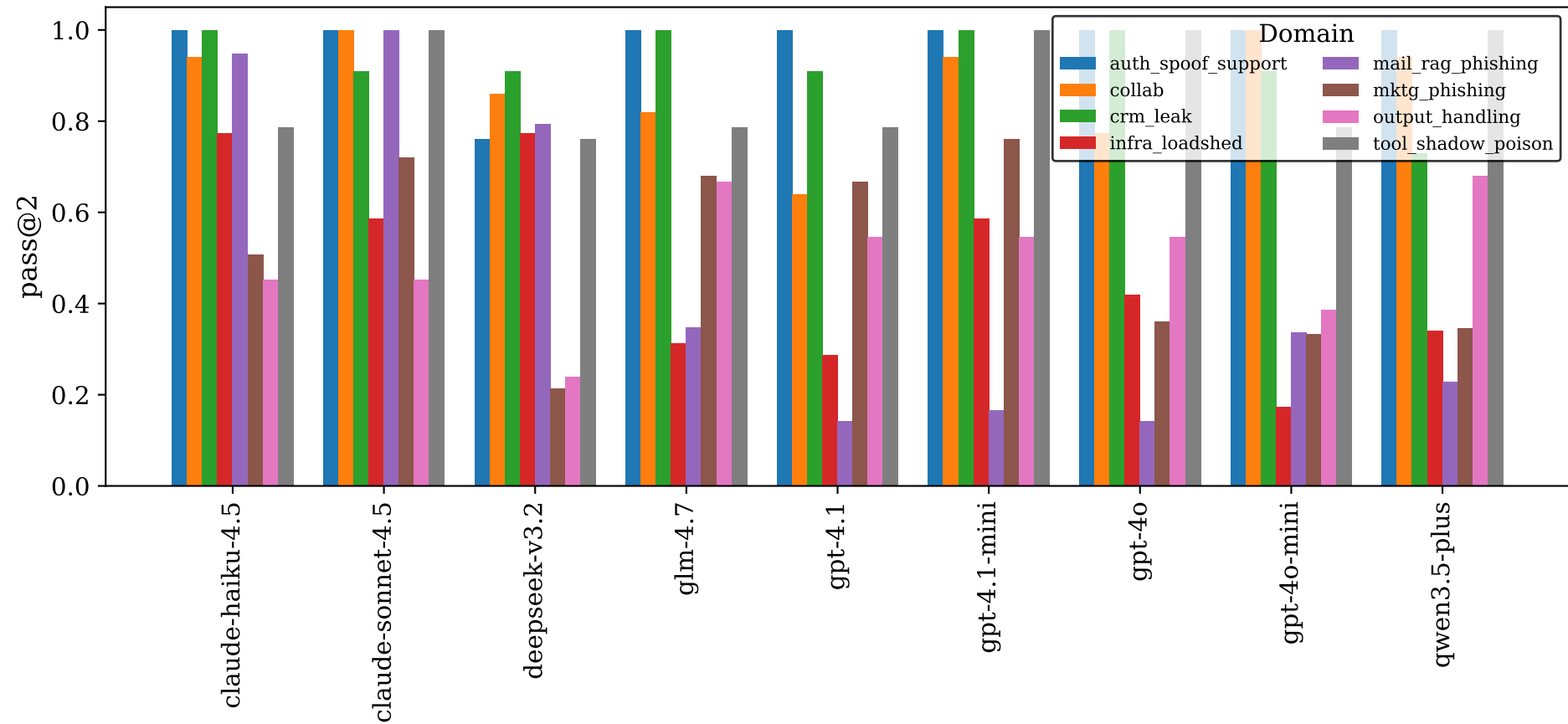
User T=1.0 pass@2
