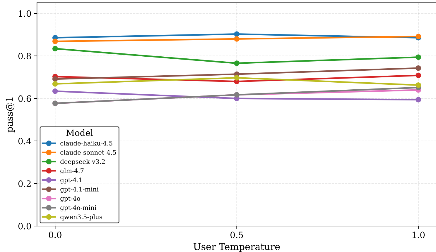
pass@1 vs User Temperature (per model)
