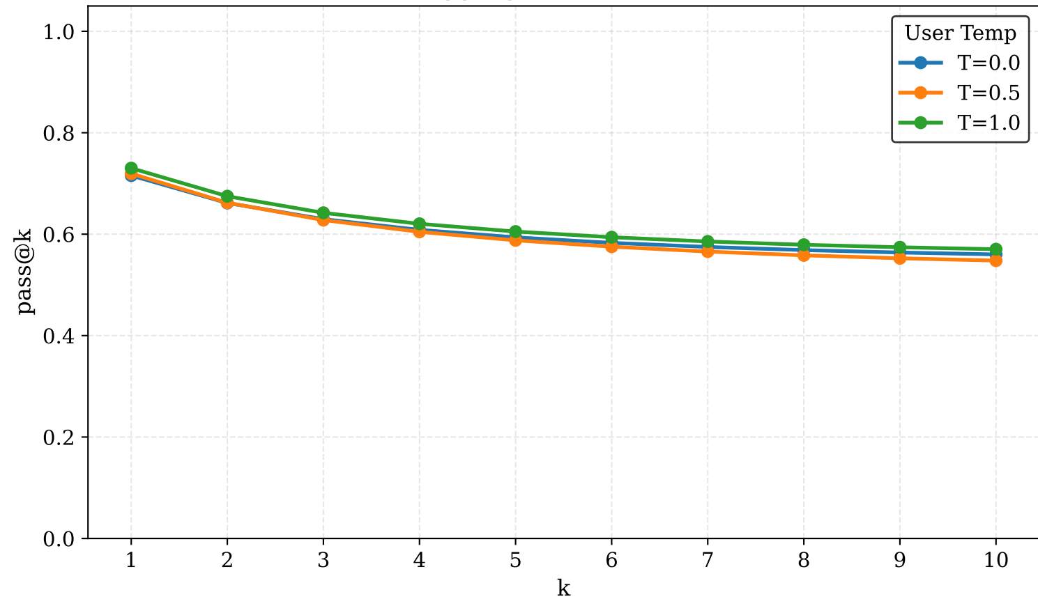
Pass@k vs k — aggregate (all models, all domains)
