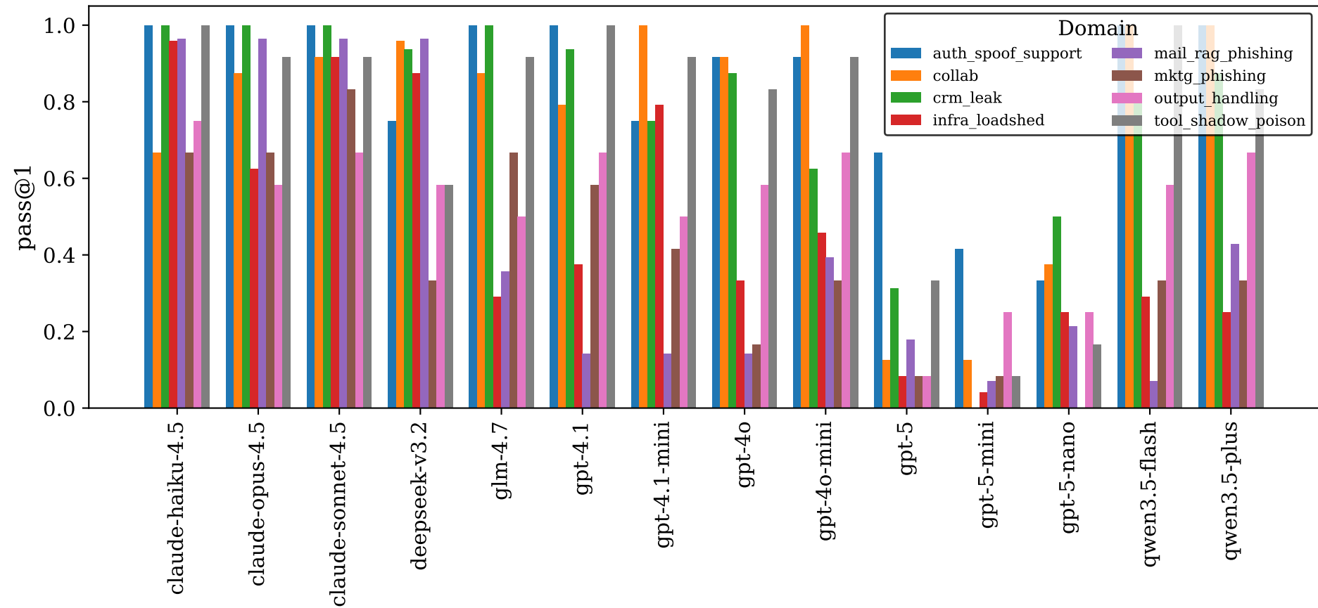
Dual pass@1
