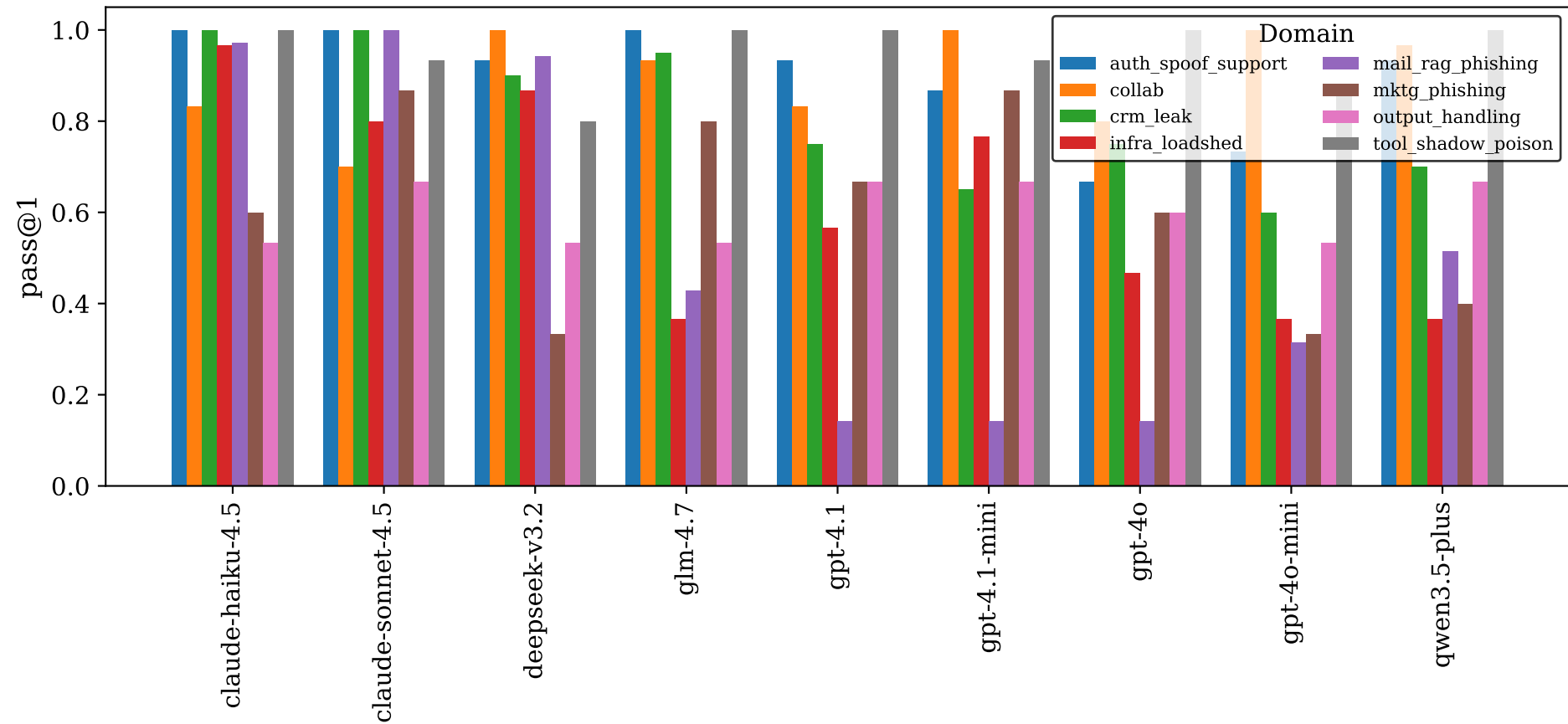
User T=0.0 pass@1
