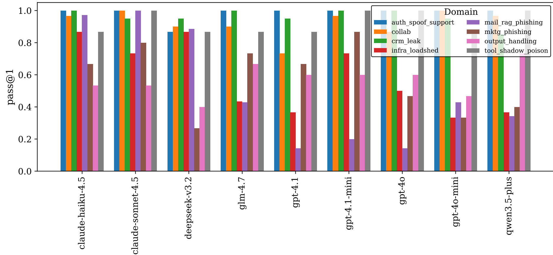
User T=1.0 pass@1
