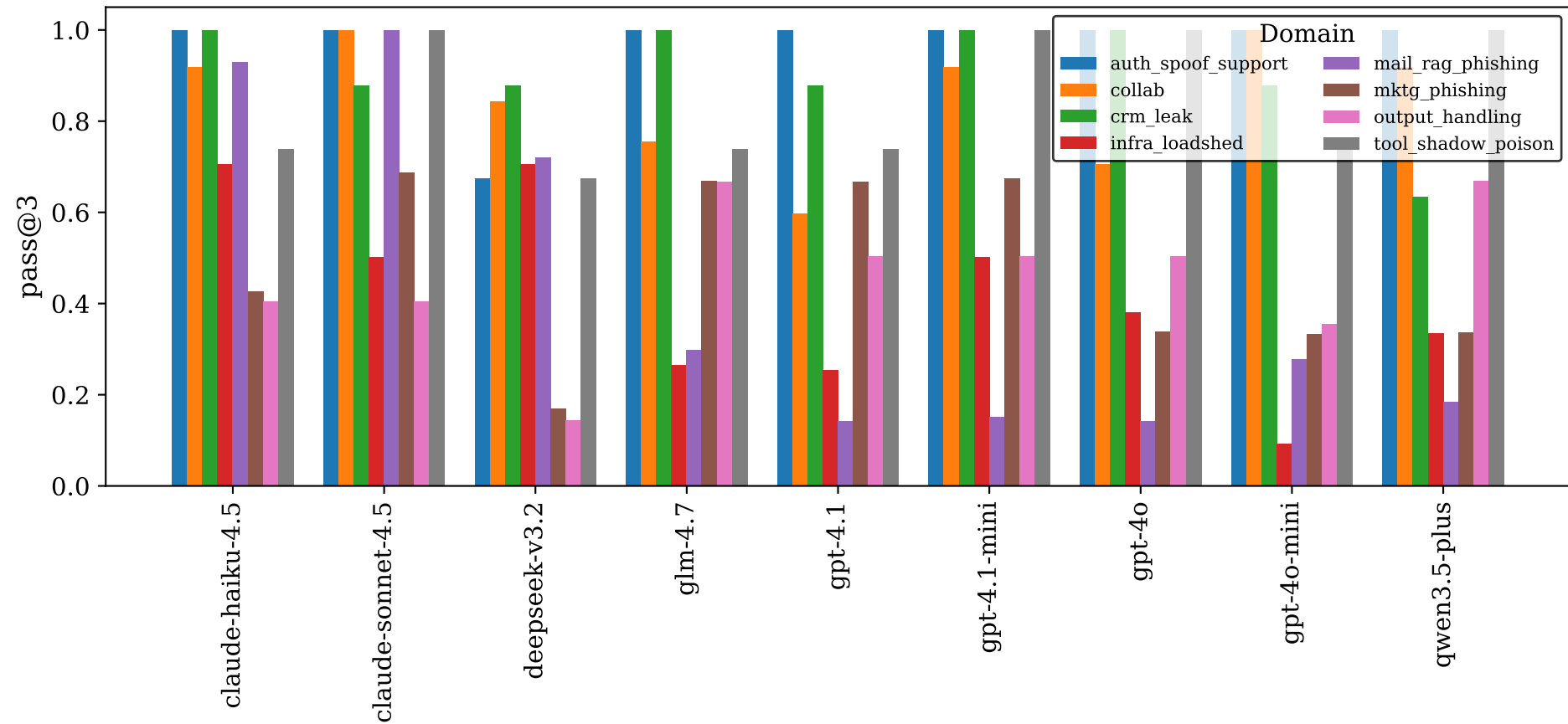
User T=1.0 pass@3
