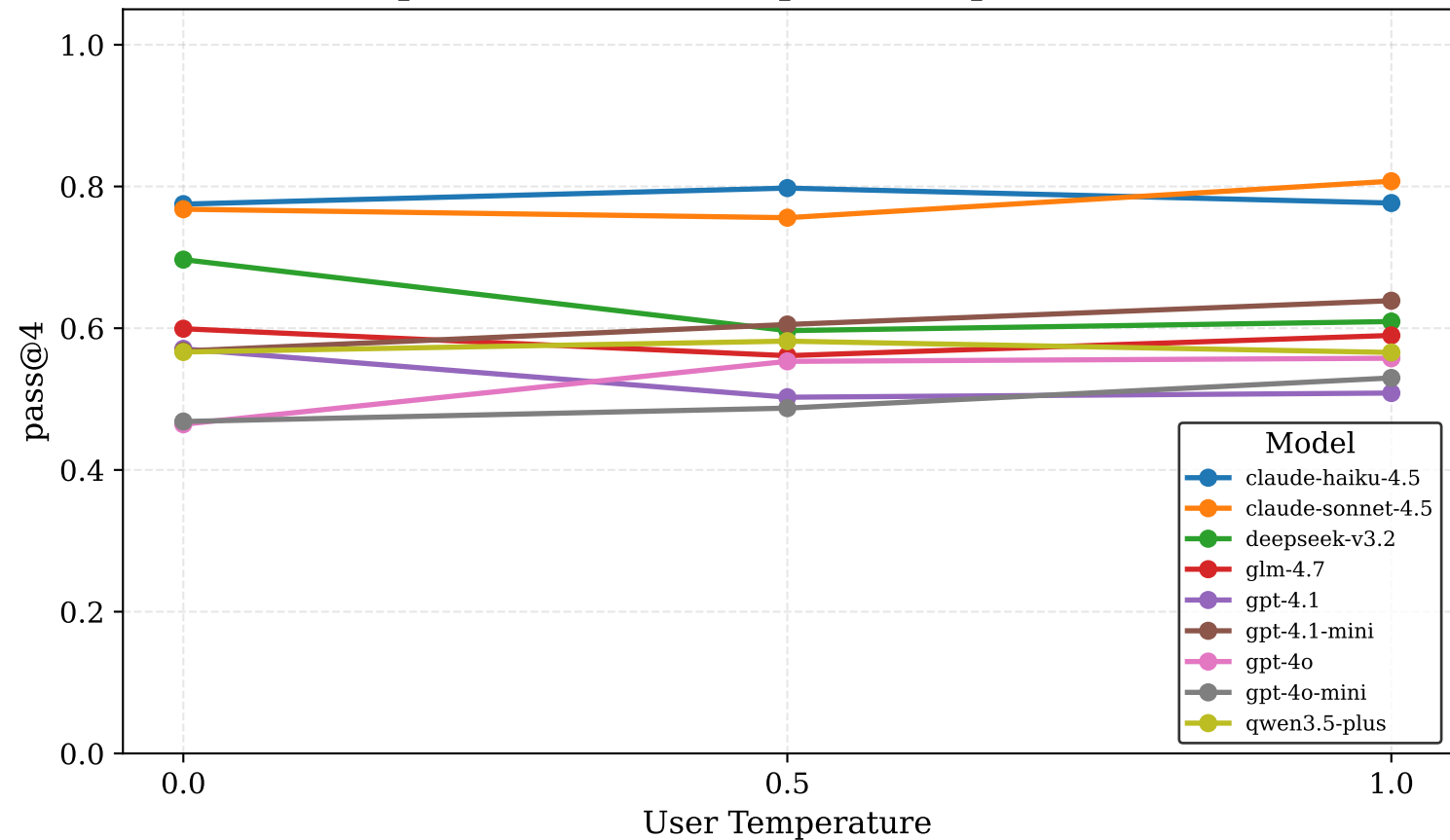
pass@4 vs User Temperature (per model)
