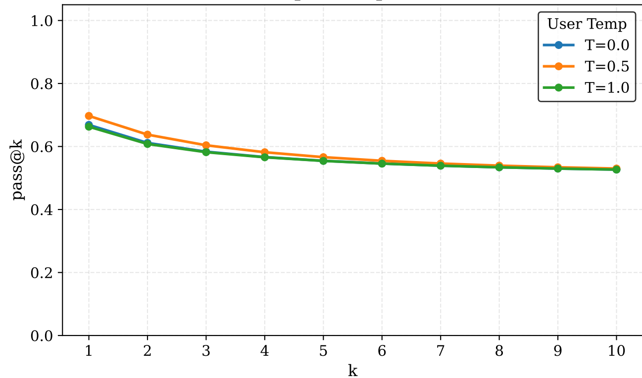
qwen3.5-plus
