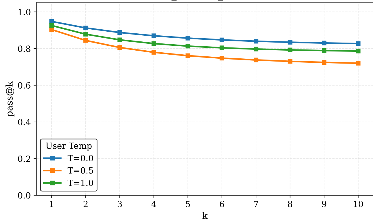
tool_shadow_poison
