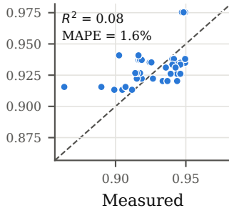
Accuracy
